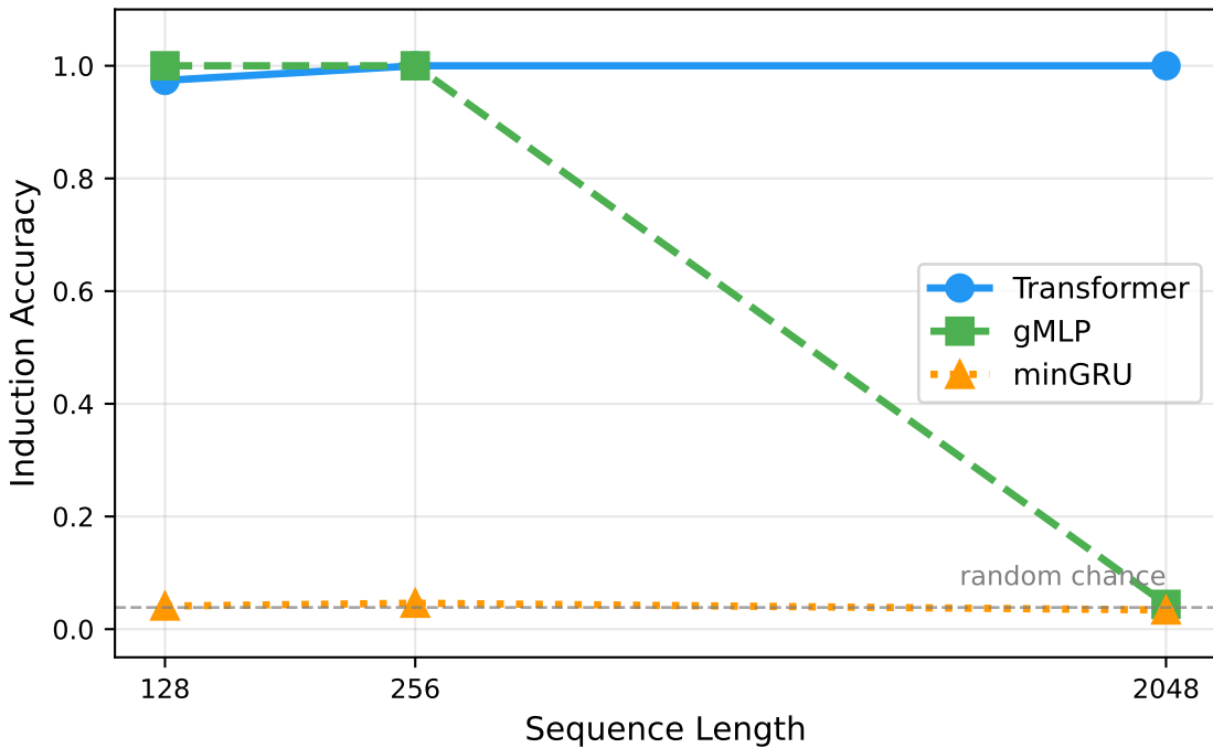
Induction Head Task — Accuracy vs. Sequence Length
