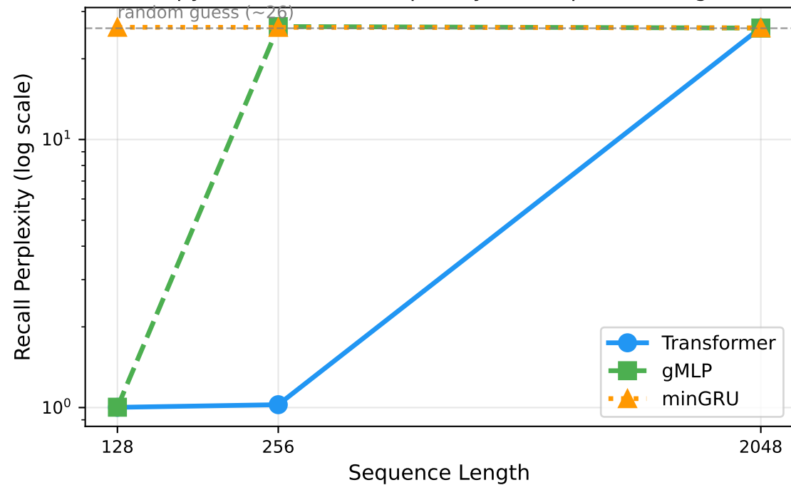
Copy Task — Recall Perplexity vs. Sequence Length
