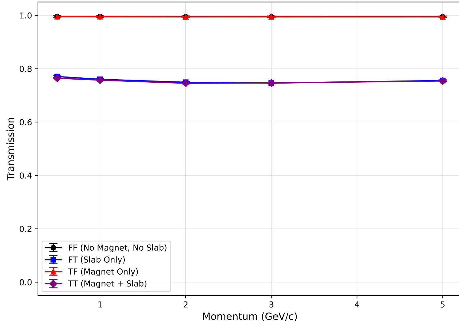
Transmission vs Momentum (Aluminum6061)
