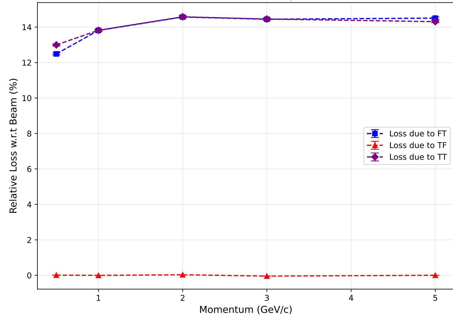
Fractional Beam Loss (Polycarbonate)
