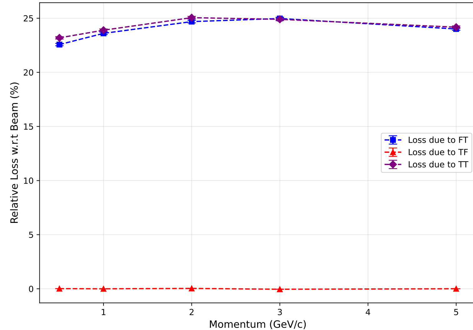
Fractional Beam Loss (Aluminum6061)
