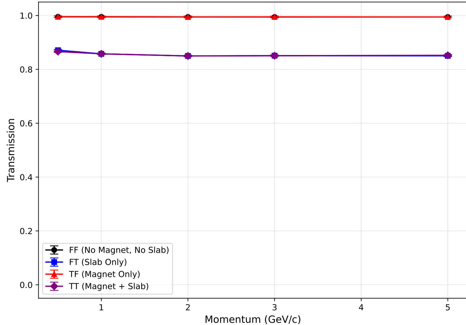
Transmission vs Momentum (Polycarbonate)
