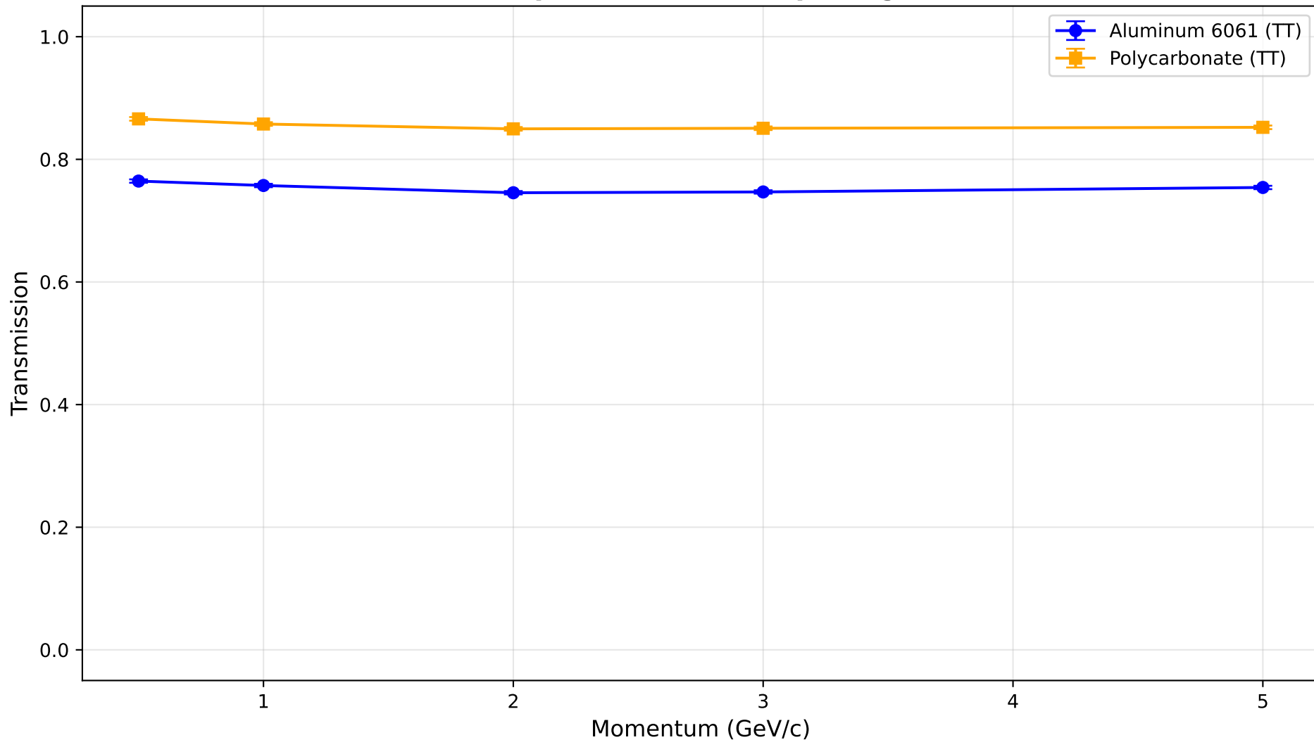
Material Comparison: Full Setup (Magnet + Slab)
