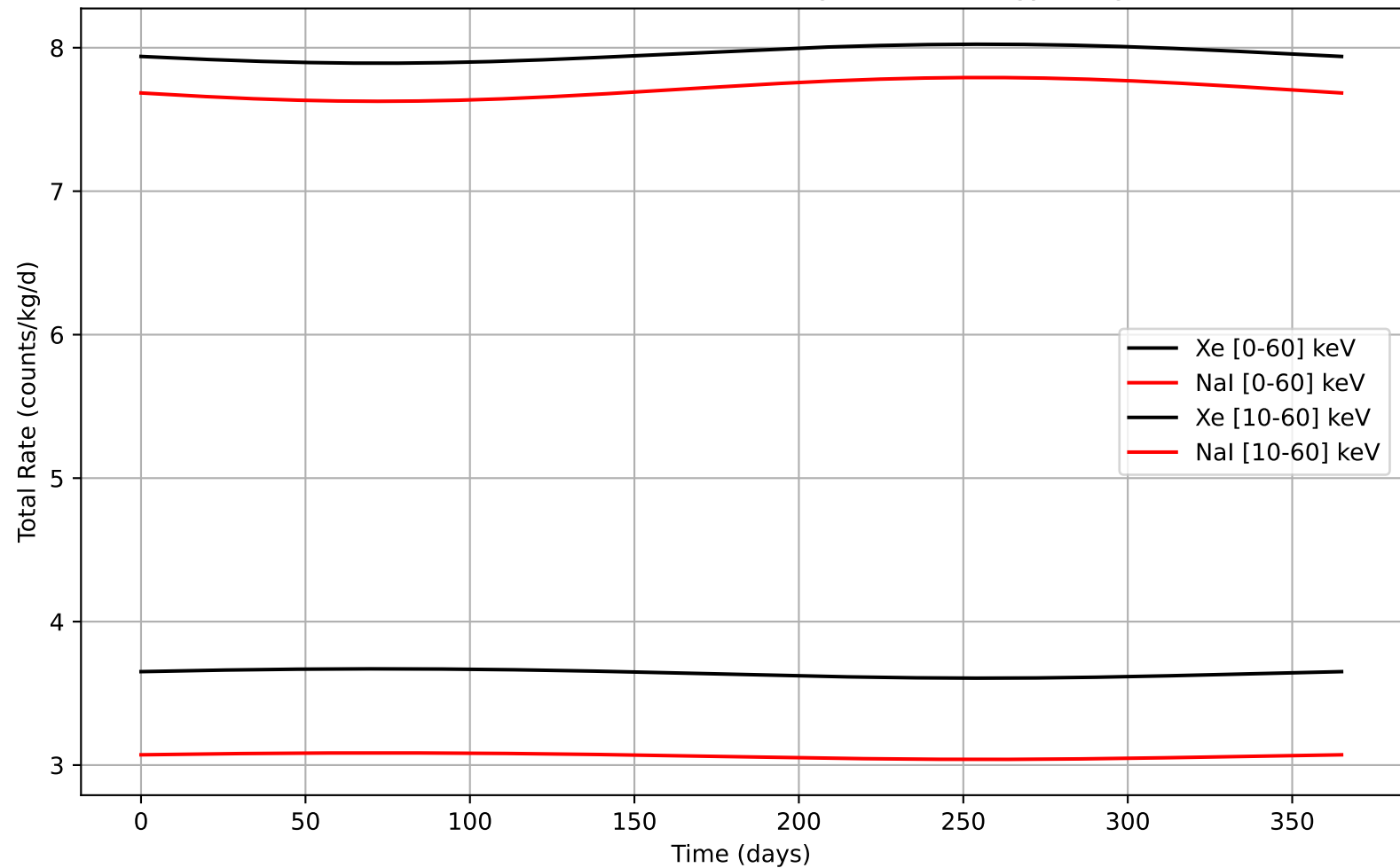
Total Rate vs Time for Different Targets and Energy Ranges
