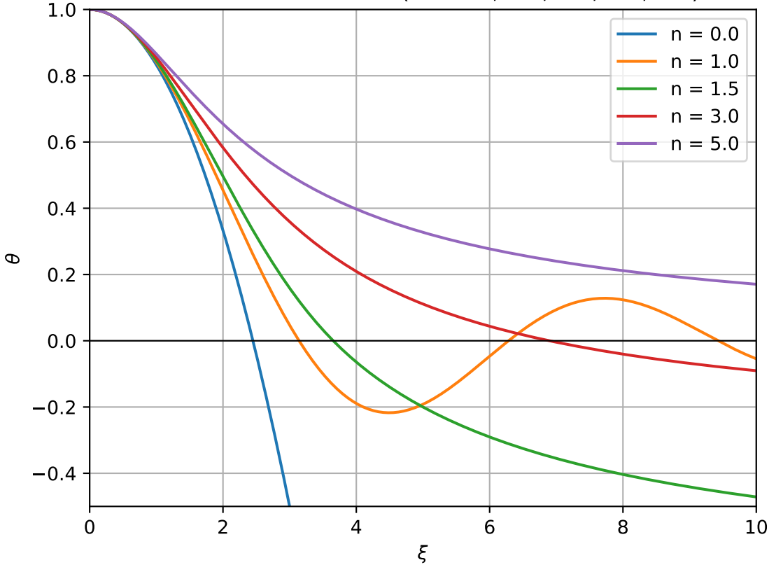
Lane-Emden solutions ( n = 0.0, 1.0, 1.5, 3.0, 5.0 )
