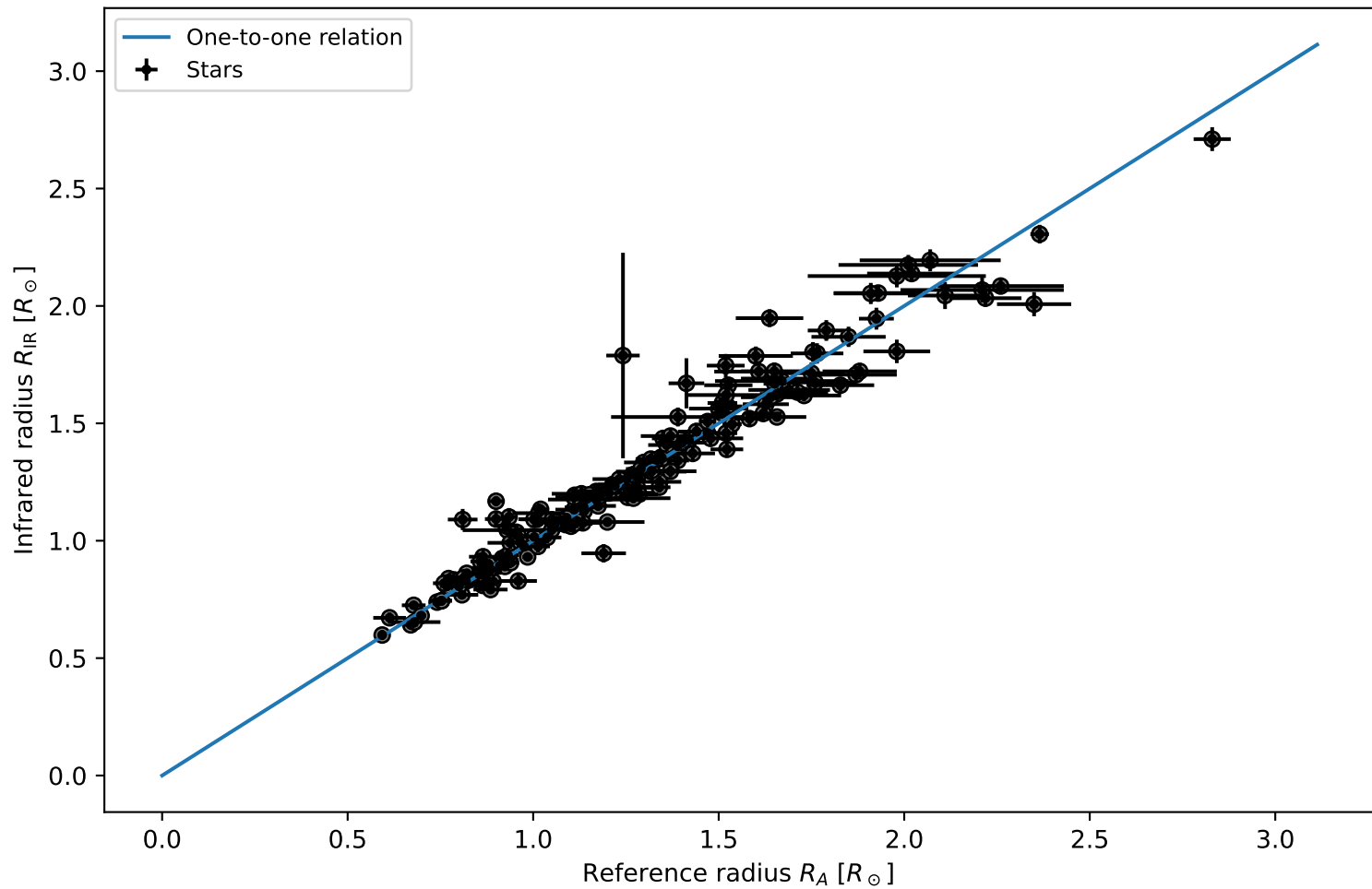
Final infrared radius comparison
