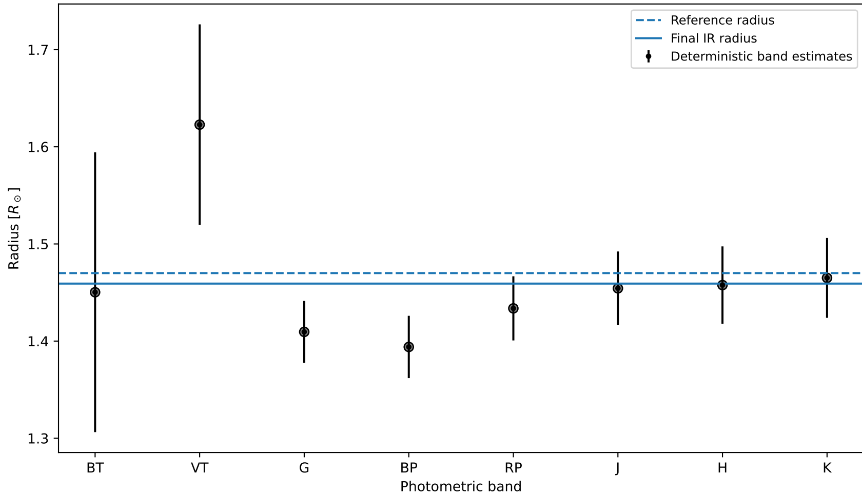
Multi-band radius estimates: WASP-001
