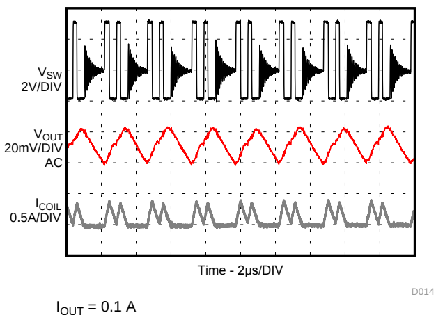
Figure 15. Power Save Mode Operation
