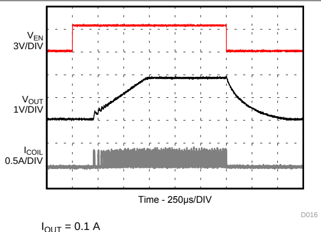
Figure 17. Startup with Load
