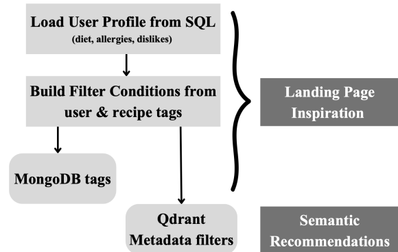
Figure 2: Recommendation Pipeline
