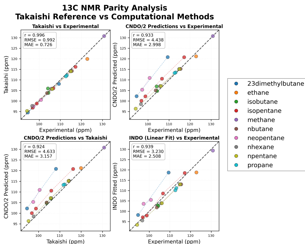
Figure 2. Parity Plots of ^{13}\text{C} NRM spectra
