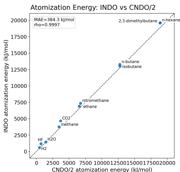
Figure 1. Parity Plots of Atomization Energies for CNDO/2 and INDO methods
