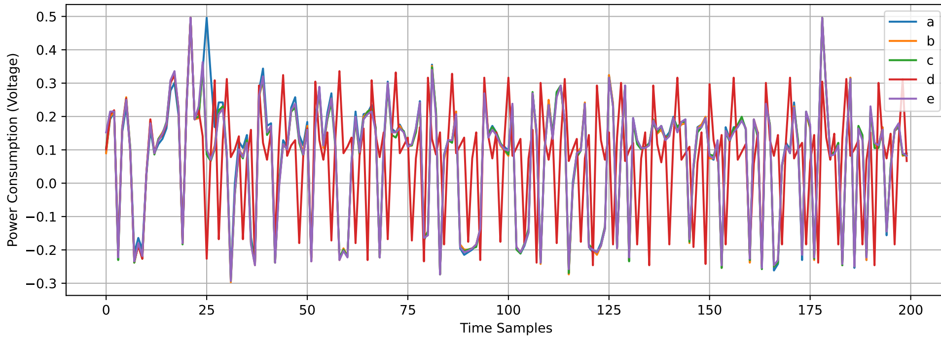
Power Consumption Traces for Different Input Characters
