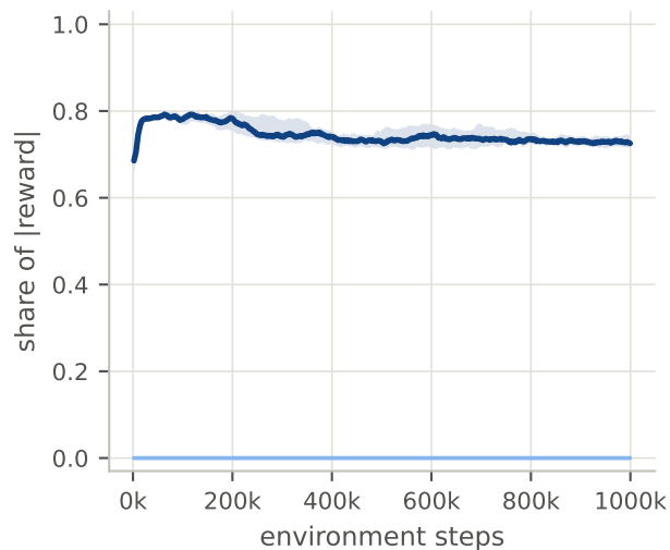
(f) Extrinsic share of the worker's reward
