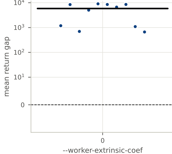
(h) Knock-out: mirrored goal
