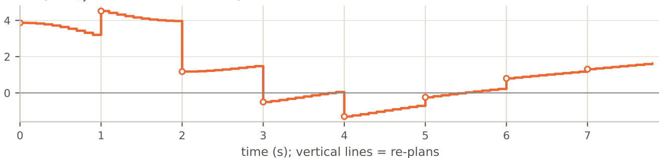
(c) goal g_y (m), relative to the agent
