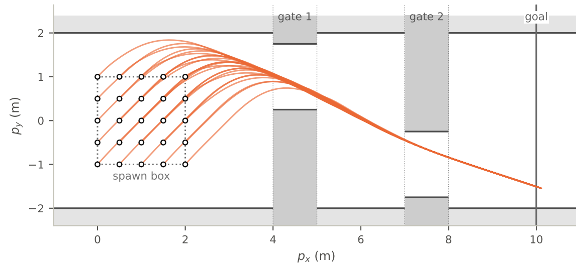
hPPO, seed 6 (final.pt), same starts: 25/25 reach the goal, +1.0 steps vs the oracle on average, 0 contacts
