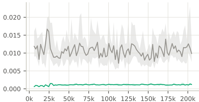
PPO+MPC: centred L2-discrepancy, last 32 starts
