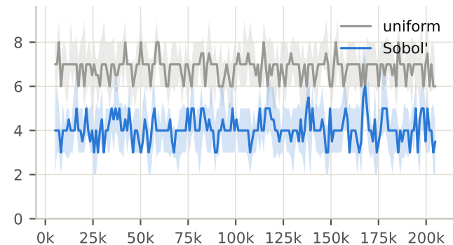
hPPO: empty 5x5 cells, last 32 starts
