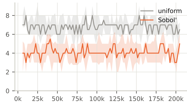
PPO+MPC: empty 5x5 cells, last 32 starts
