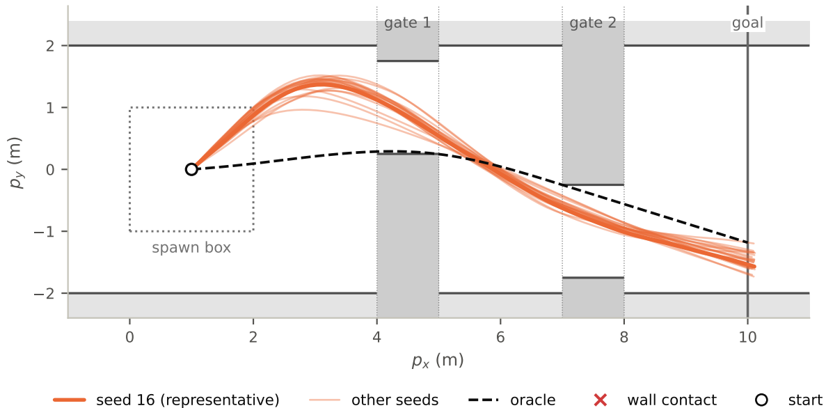
hPPO, Sobol', all 20 seeds from (1.0, 0.0): 20 reach the goal, 79-79 steps (oracle 78)
