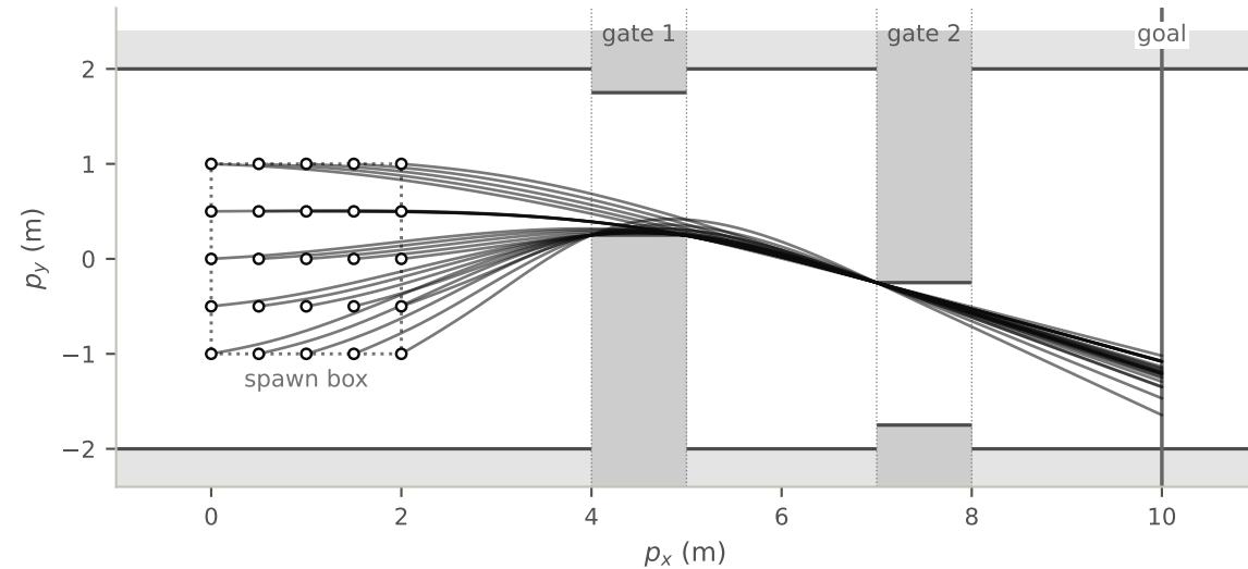
hPPO, Sobol', seed 16 (final.pt), same starts: 25/25 reach the goal, +0.7 steps vs the oracle on average, 0 contacts
