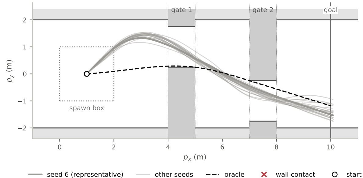
hPPO, uniform, all 20 seeds from (1.0, 0.0): 20 reach the goal, 79-79 steps (oracle 78)
