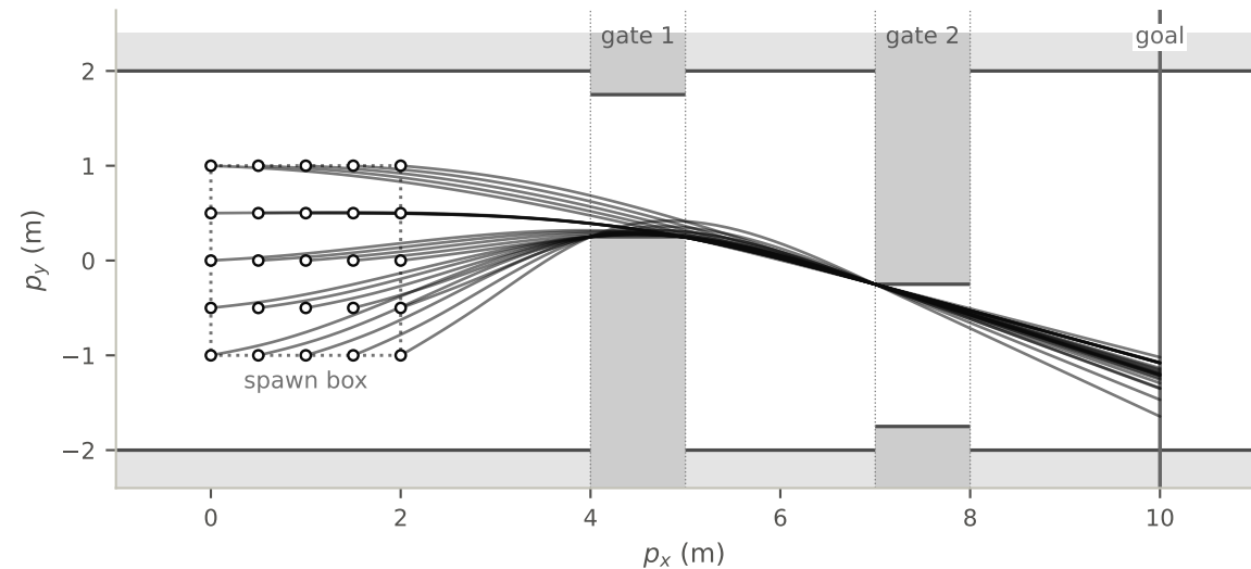
hPPO, uniform, seed 6 (final.pt), same starts: 25/25 reach the goal, +1.0 steps vs the oracle on average, 0 contacts
