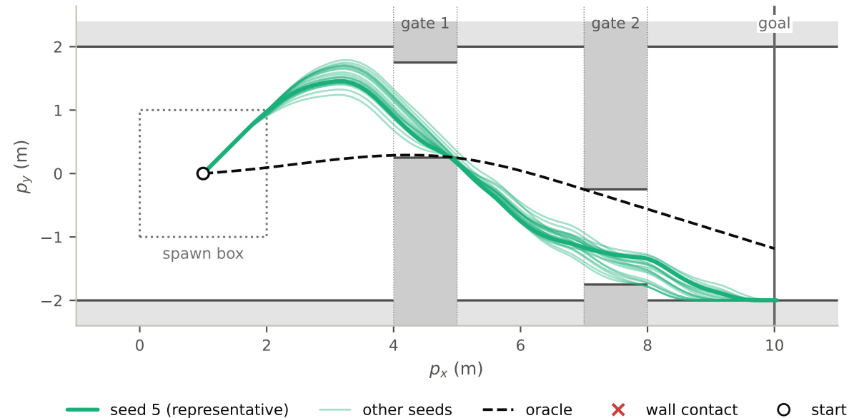
PPO+MPC, Sobol', all 20 seeds from (1.0, 0.0): 20 reach the goal, 78-78 steps (oracle 78)
