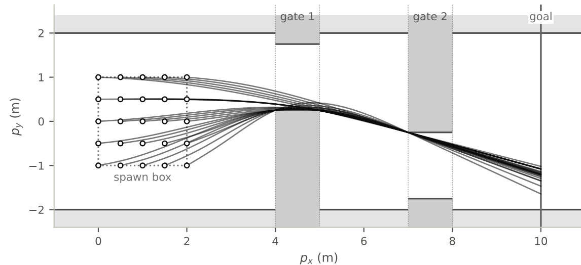
PPO+MPC, Sobol', seed 5 (final.pt), same starts: 25/25 reach the goal, +0.2 steps vs the oracle on average, 0 contacts
