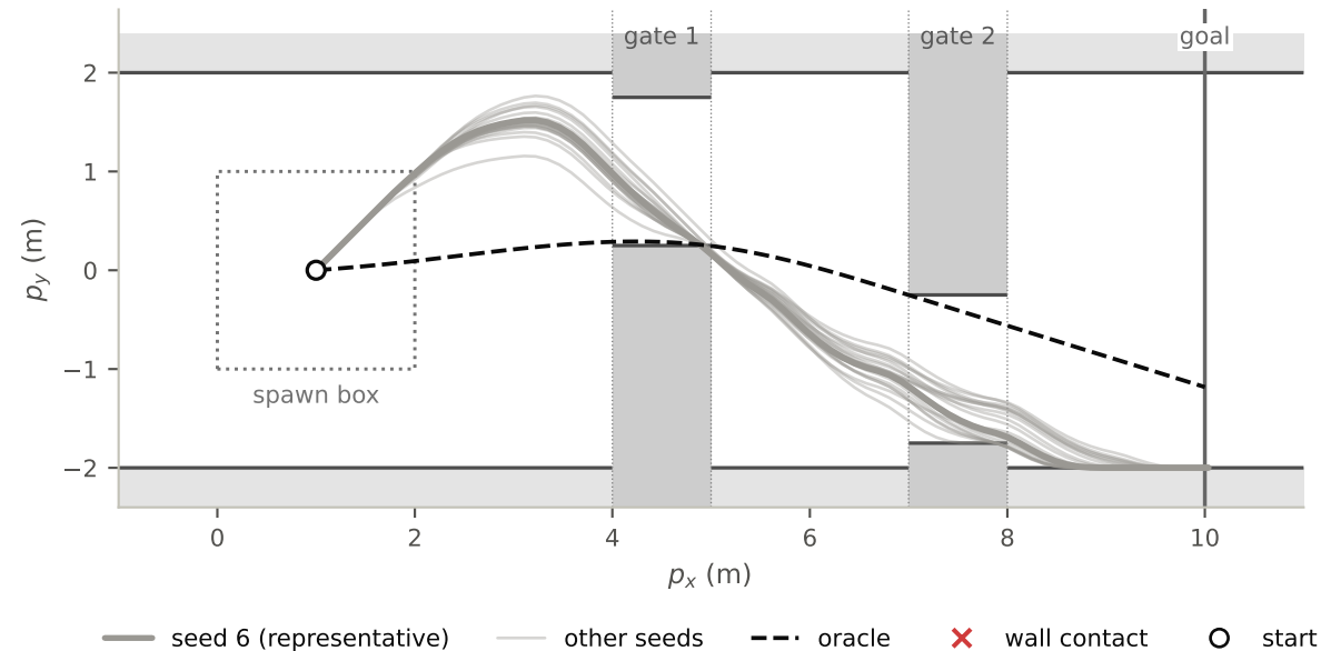
PPO+MPC, uniform, all 20 seeds from (1.0, 0.0): 20 reach the goal, 78-78 steps (oracle 78)
