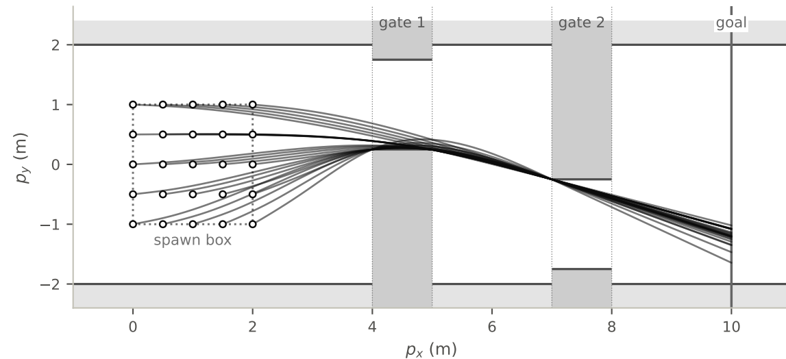
PPO+MPC, uniform, seed 6 (final.pt), same starts: 25/25 reach the goal, +0.2 steps vs the oracle on average, 0 contacts
