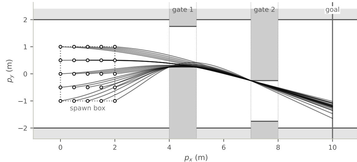
PPO, Sobol', seed 4 (final.pt), same starts: 25/25 reach the goal, +0.2 steps vs the oracle on average, 0 contacts
