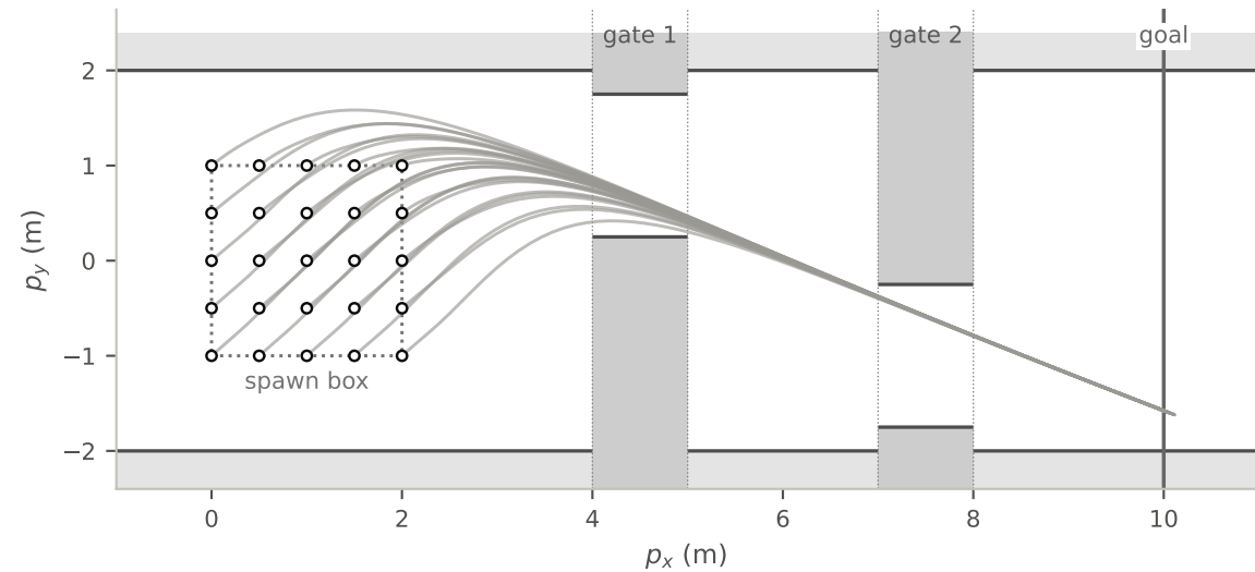
PPO, uniform, seed 6 (final.pt), same starts: 25/25 reach the goal, +0.2 steps vs the oracle on average, 0 contacts
