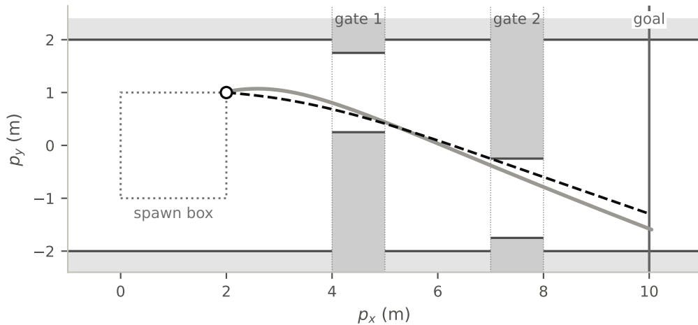
start (2.0, 1.0): PPO, uniform 70 steps; oracle 70 steps
