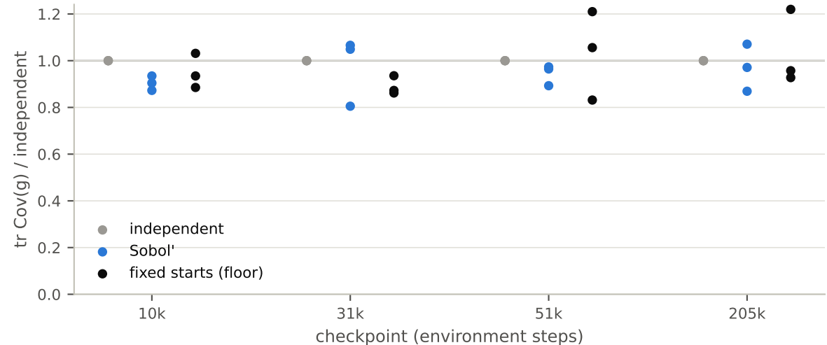
Policy-gradient variance by how the batch's starts are drawn (flat PPO, slalom)
