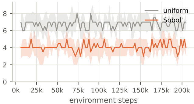
hPPO: empty 5x5 cells, last 32 starts
