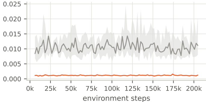
hPPO: centred L2-discrepancy, last 32 starts
