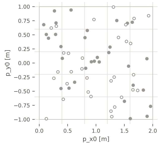
uniform 9 empty cells after 32 starts, 2 after 64
