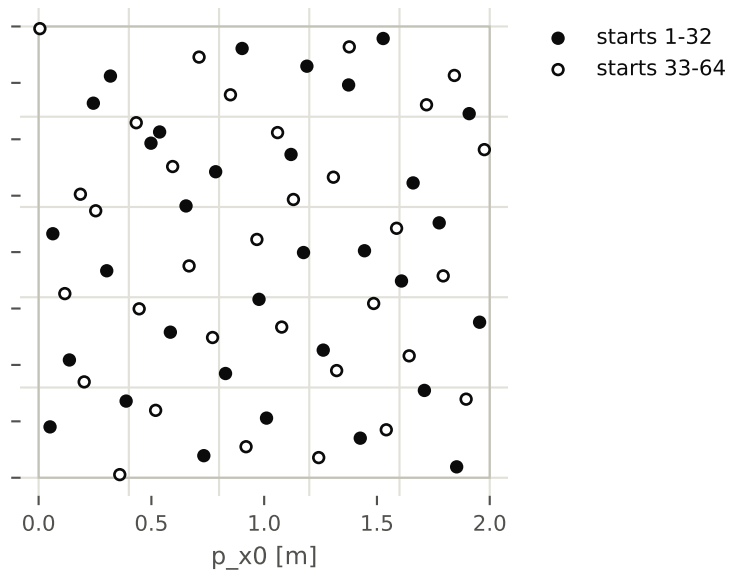
Sobol' 4 empty cells after 32 starts, 0 after 64
