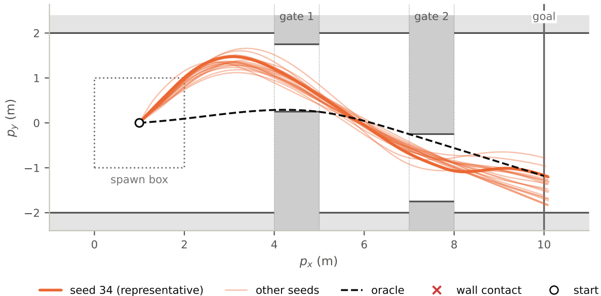
hPPO, Sobol', all 20 seeds from (1.0, 0.0): 20 reach the goal, 79-80 steps (oracle 78)
