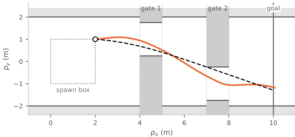
start (2.0, 1.0): hPPO, Sobol' 71 steps; oracle 70 steps
