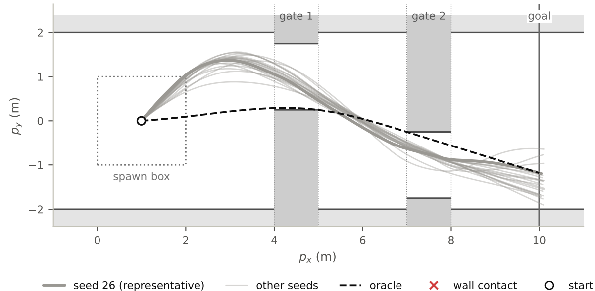
hPPO, uniform, all 20 seeds from (1.0, 0.0): 20 reach the goal, 78-80 steps (oracle 78)
