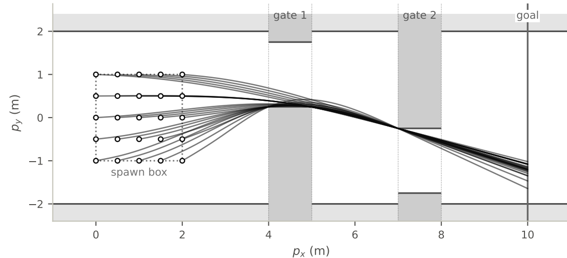
hPPO, uniform, seed 26 (final.pt), same starts: 25/25 reach the goal, +1.2 steps vs the oracle on average, 0 contacts
