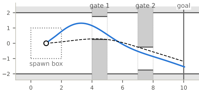
205k steps (end): 78 steps
