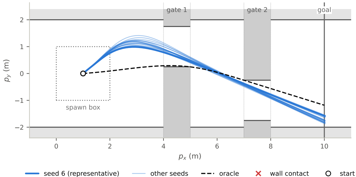
PPO, all 20 seeds from (1.0, 0.0): 20 reach the goal, 78-78 steps (oracle 78)
