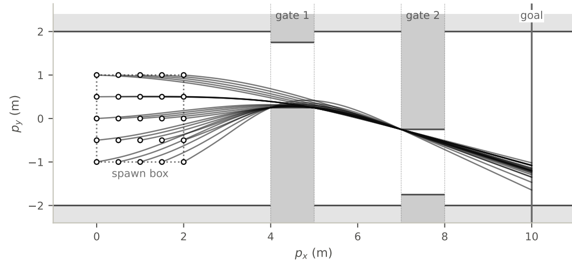
PPO, seed 6 (final.pt), same starts: 25/25 reach the goal, +0.2 steps vs the oracle on average, 0 contacts
