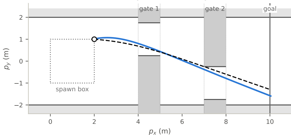
start (2.0, 1.0): PPO 70 steps; oracle 70 steps
