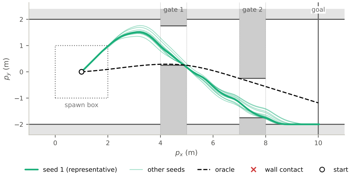
PPO+MPC, all 10 seeds from (1.0, 0.0): 10 reach the goal, 78-78 steps (oracle 78)
