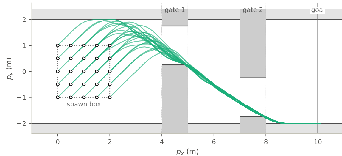
PPO+MPC, seed 1 (final.pt), same starts: 25/25 reach the goal, +0.2 steps vs the oracle on average, 0 contacts
