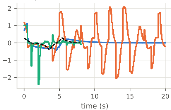
(e) a_y (m/s 2 )
