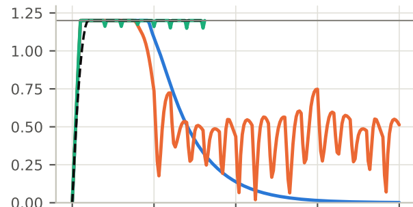
(c) speed \|v\| (m/s)
