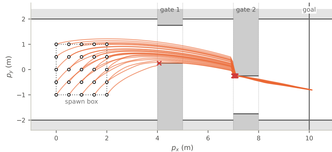
hPPO, seed 11 (final.pt), same starts: 25/25 reach the goal, +2.1 steps vs the oracle on average, 26 contacts
