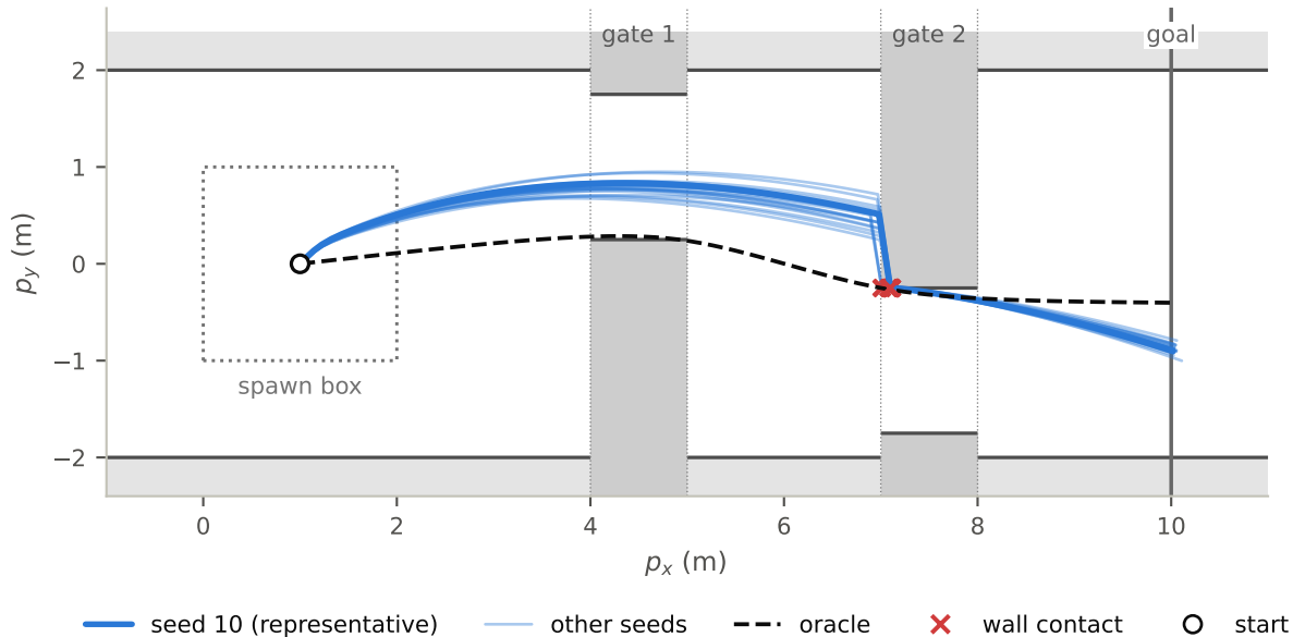
PPO, all 20 seeds from (1.0, 0.0): 20 reach the goal, 80-81 steps (oracle 79)
