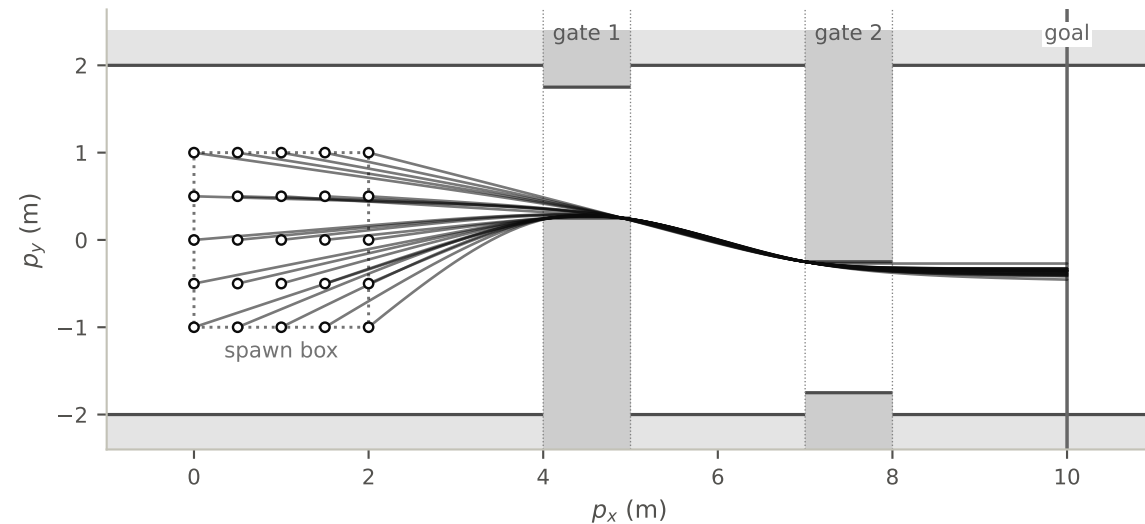
PPO+MPC, Sobol', seed 12 (final.pt), same starts: 25/25 reach the goal, +1.4 steps vs the oracle on average, 0 contacts
