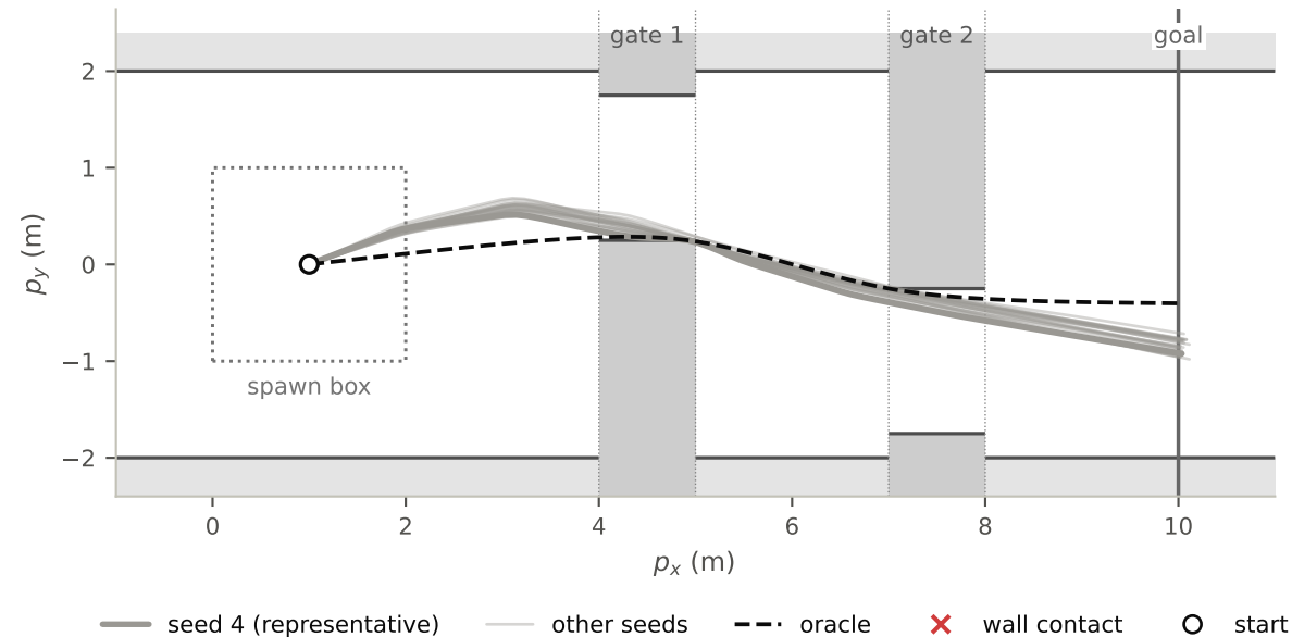
PPO+MPC, uniform, all 20 seeds from (1.0, 0.0): 20 reach the goal, 80-81 steps (oracle 79)
