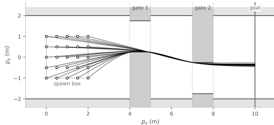
PPO+MPC, uniform, seed 4 (final.pt), same starts: 25/25 reach the goal, +1.3 steps vs the oracle on average, 0 contacts
