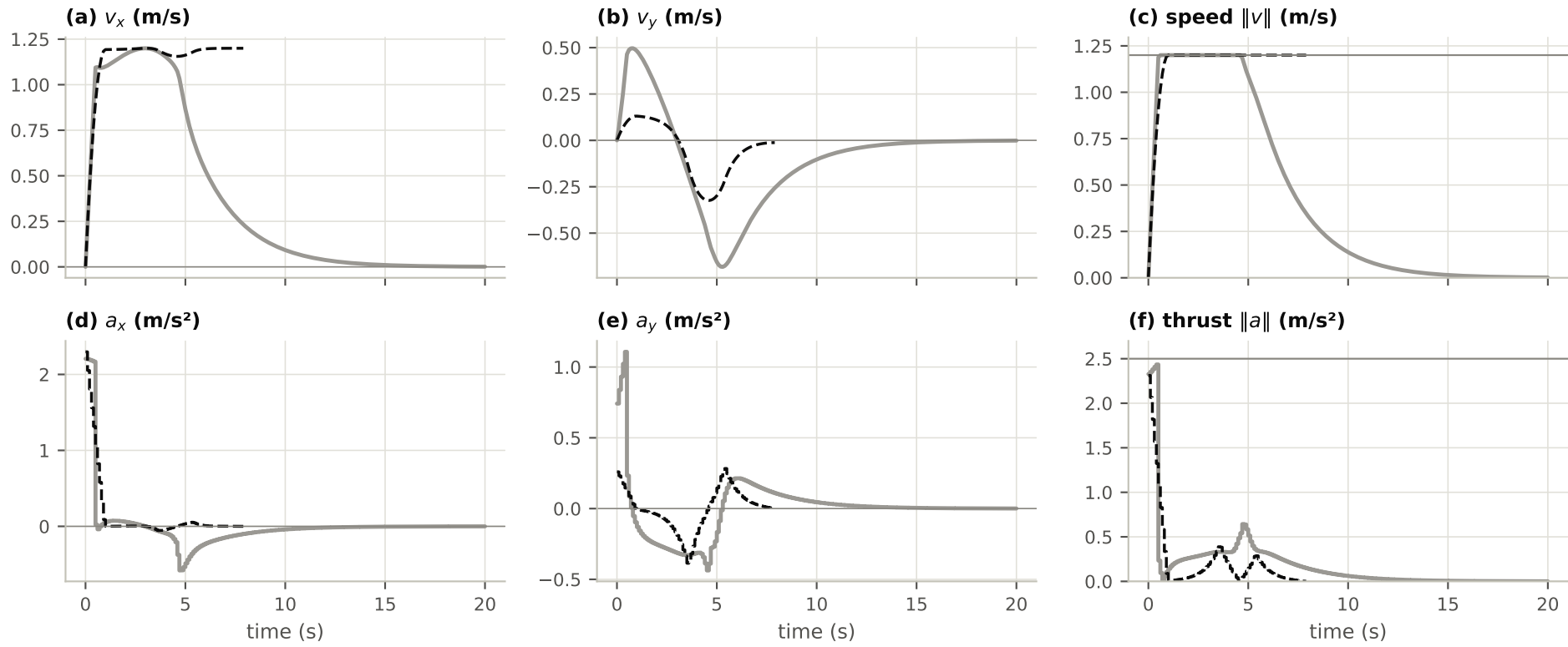
— PPO, uniform - - - oracle — limits v_{max}, u_{max}
