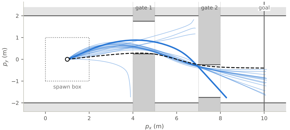
PPO, all 20 seeds from (1.0, 0.0): 14 reach the goal, 80-83 steps (oracle 79)
