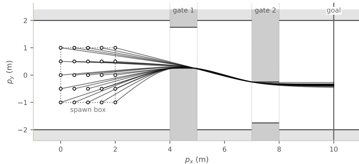
PPO+MPC, seed 1 (final.pt), same starts: 25/25 reach the goal, +1.5 steps vs the oracle on average, 0 contacts
