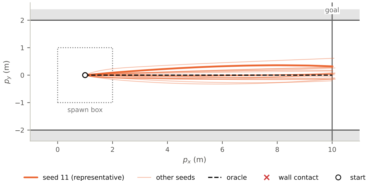
hPPO, all 20 seeds from (1.0, 0.0): 20 reach the goal, 78-79 steps (oracle 78)
